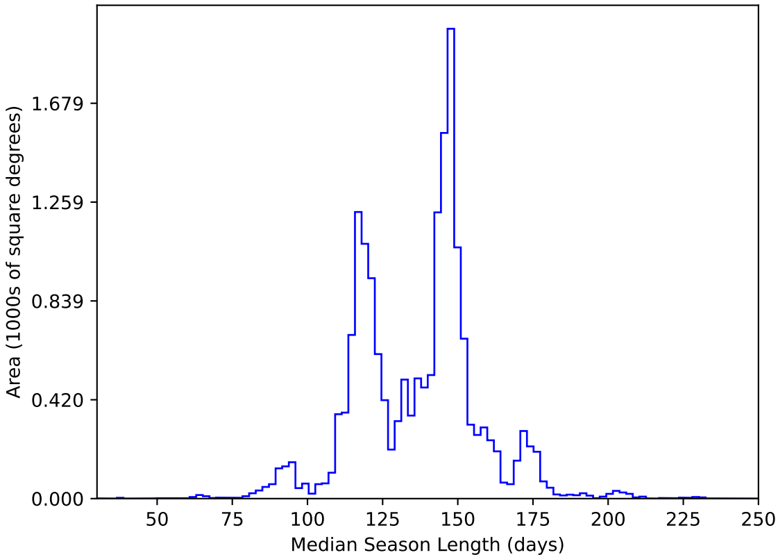
too_ignore_5_4v3.4_10yrs WFD y band: Median Season Length
