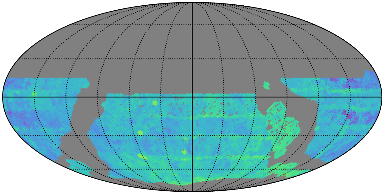
too_ignore_5_4v3.4_10yrs WFD r band: Median Season Length
