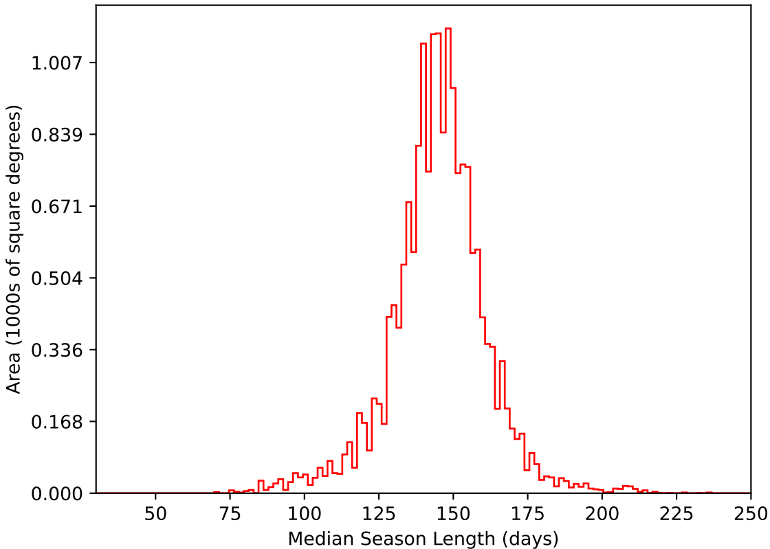
too_ignore_5_4v3.4_10yrs WFD i band: Median Season Length
