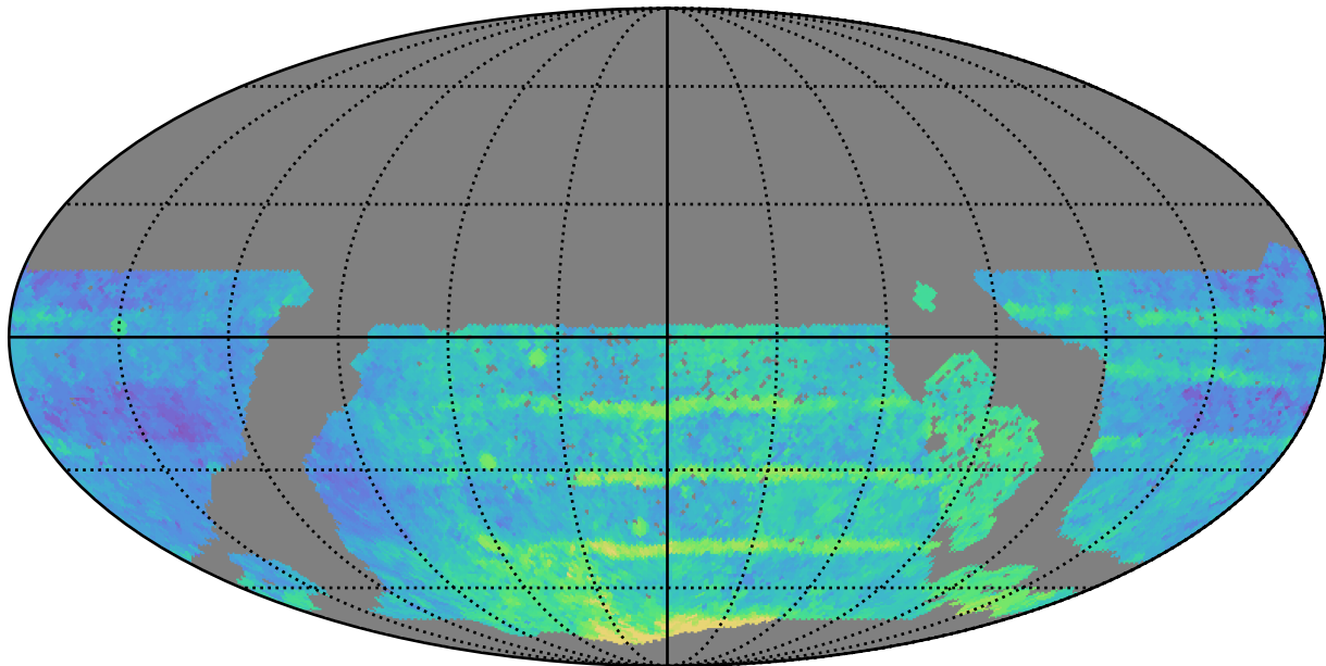
too_ignore_5_4v3.4_10yrs WFD all bands: Median Season Length
