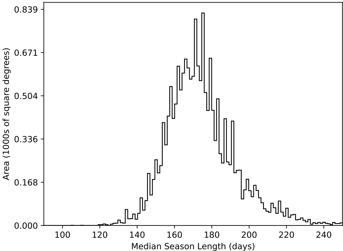
too_ignore_5_4v3.4_10yrs WFD all bands: Median Season Length
