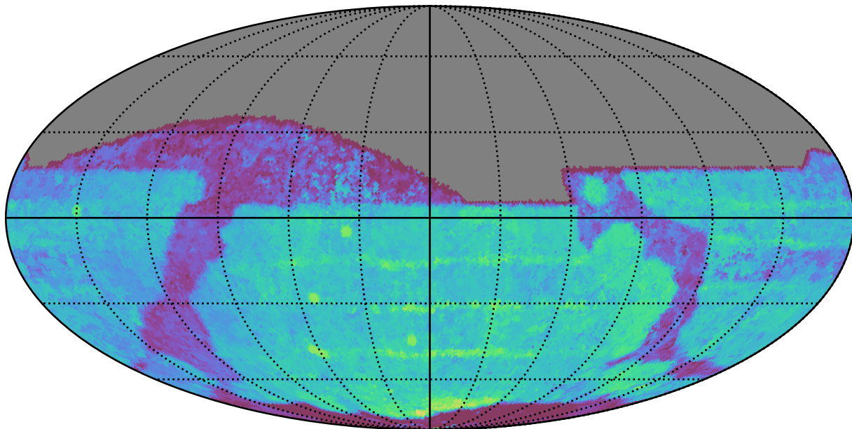
too_ignore_5_4v3.4_10yrs All sky z band: Median Season Length
