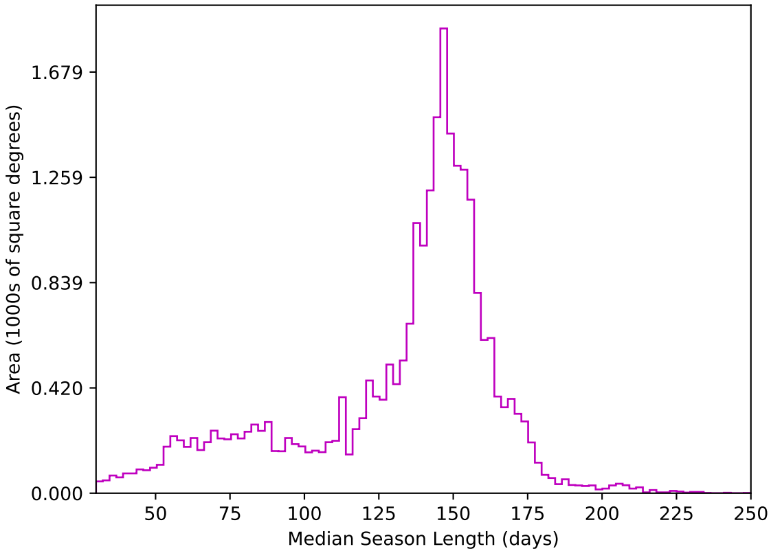
too_ignore_5_4v3.4_10yrs All sky z band: Median Season Length
