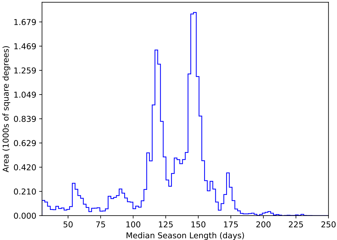
too_ignore_5_4v3.4_10yrs All sky y band: Median Season Length
