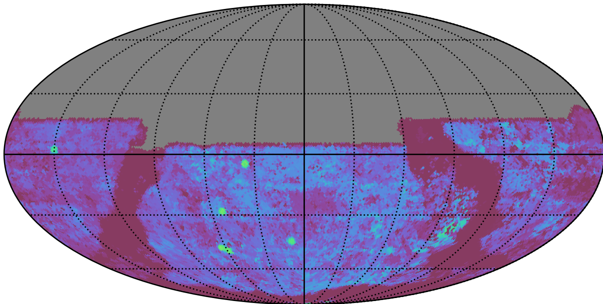
too_ignore_5_4v3.4_10yrs All sky u band: Median Season Length
