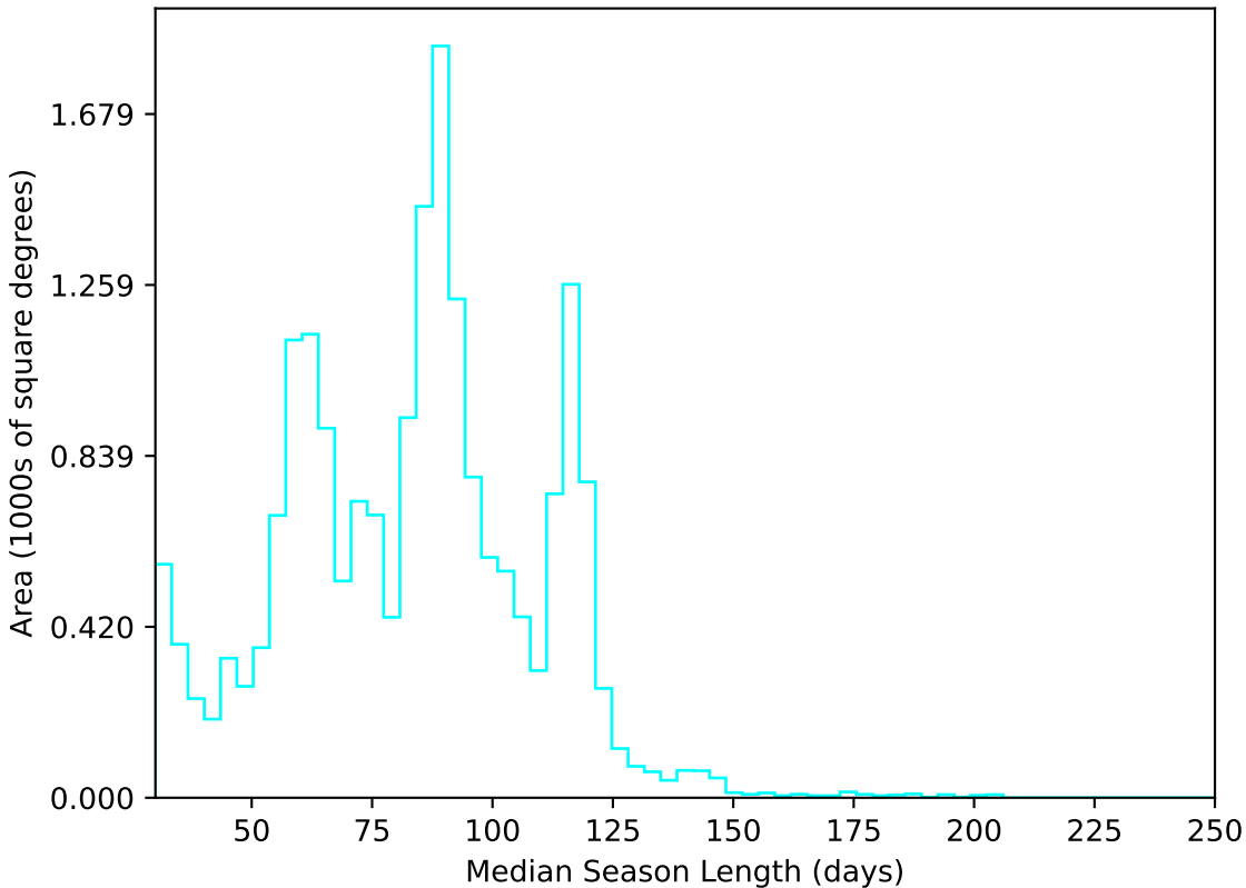
too_ignore_5_4v3.4_10yrs All sky u band: Median Season Length
