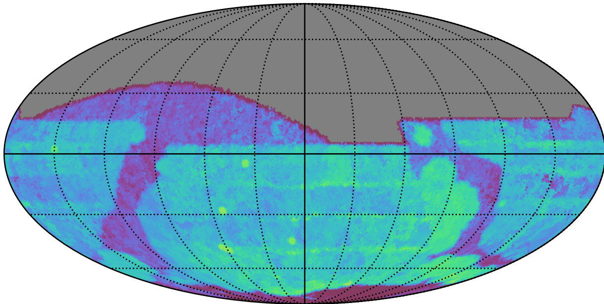
too_ignore_5_4v3.4_10yrs All sky r band: Median Season Length
