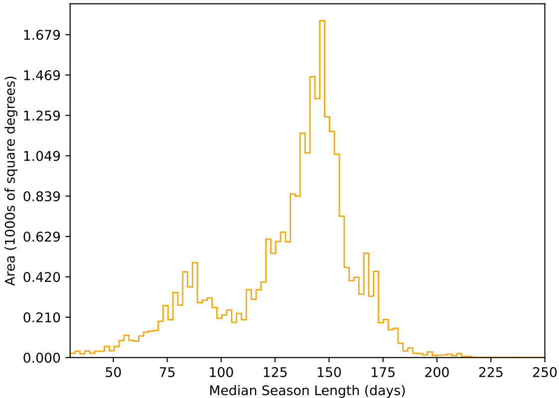
too_ignore_5_4v3.4_10yrs All sky r band: Median Season Length
