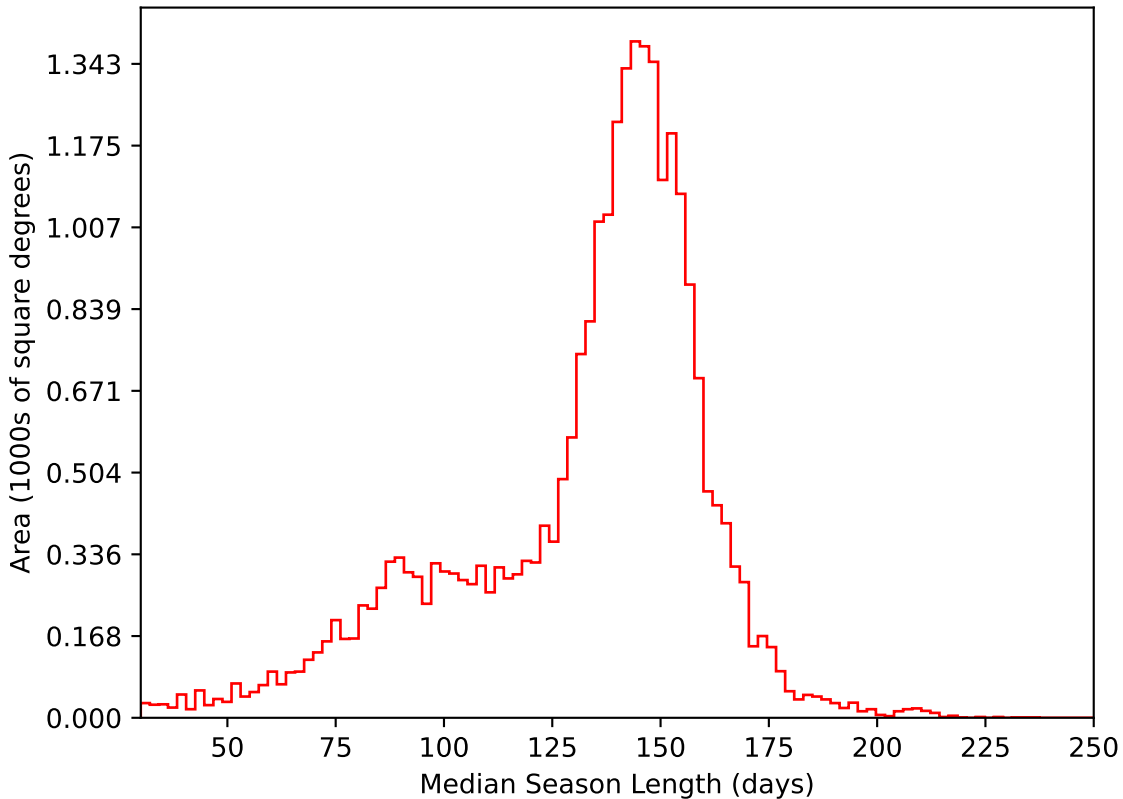
too_ignore_5_4v3.4_10yrs All sky i band: Median Season Length
