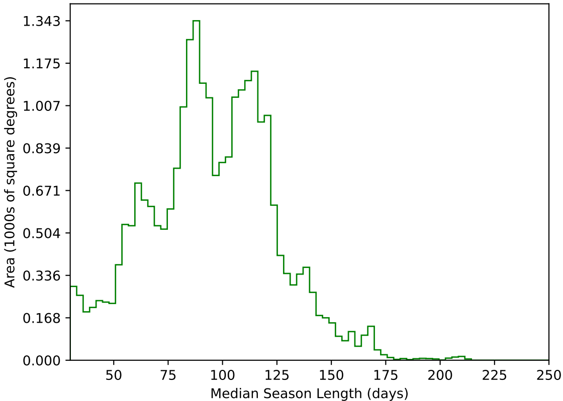
too_ignore_5_4v3.4_10yrs All sky g band: Median Season Length
