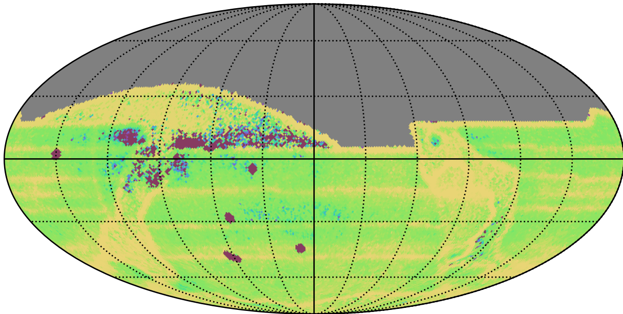
too_ignore_5_4v3.4_10yrs All sky: Median Intra-Night Gap
