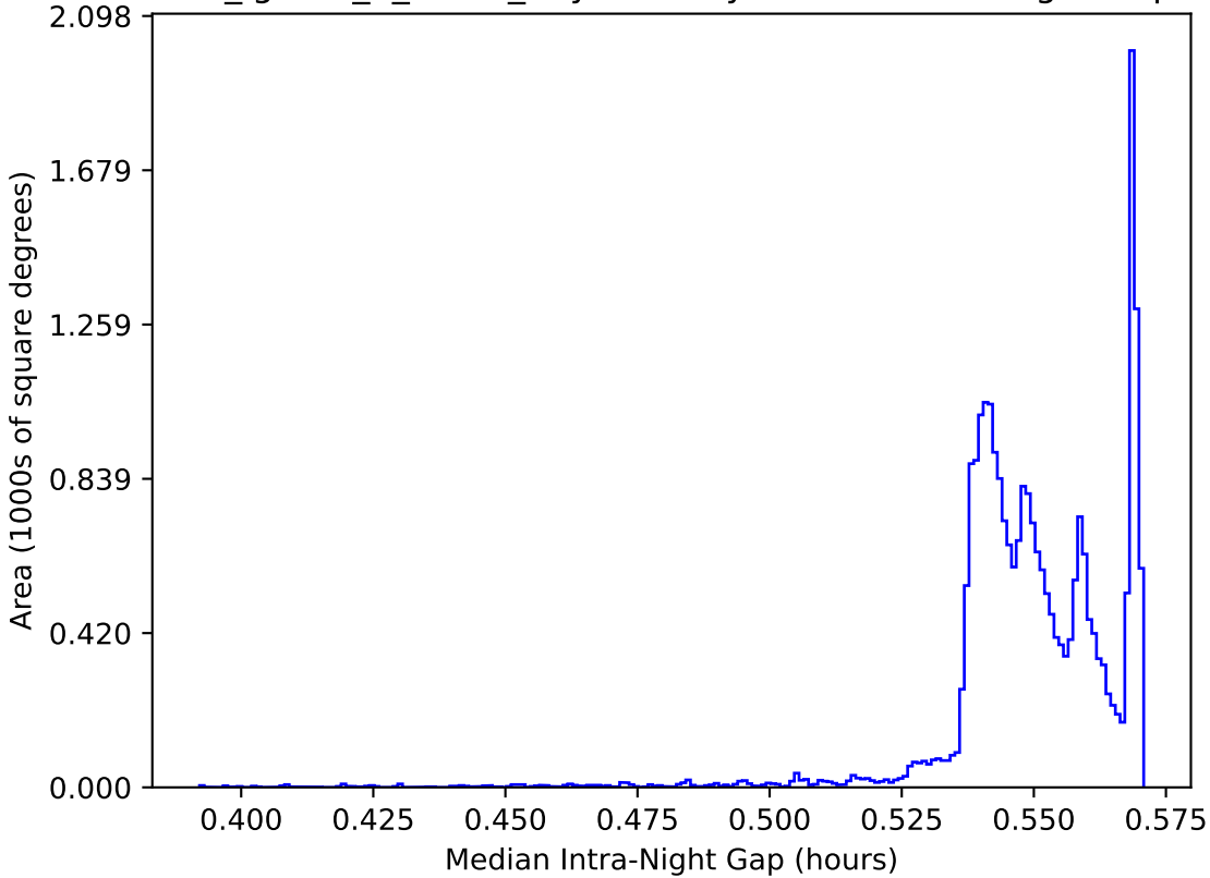
too_ignore_5_4v3.4_10yrs All sky: Median Intra-Night Gap
