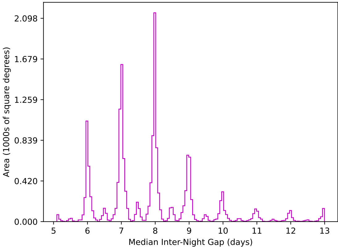
too_ignore_5_4v3.4_10yrs WFD z band: Median Inter-Night Gap
