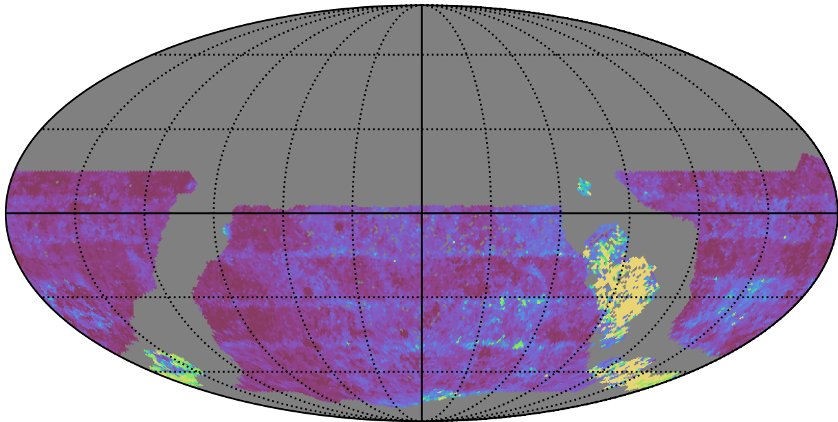
too_ignore_5_4v3.4_10yrs WFD u band: Median Inter-Night Gap
