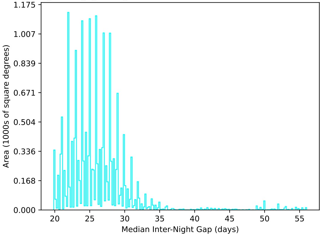
too_ignore_5_4v3.4_10yrs WFD u band: Median Inter-Night Gap
