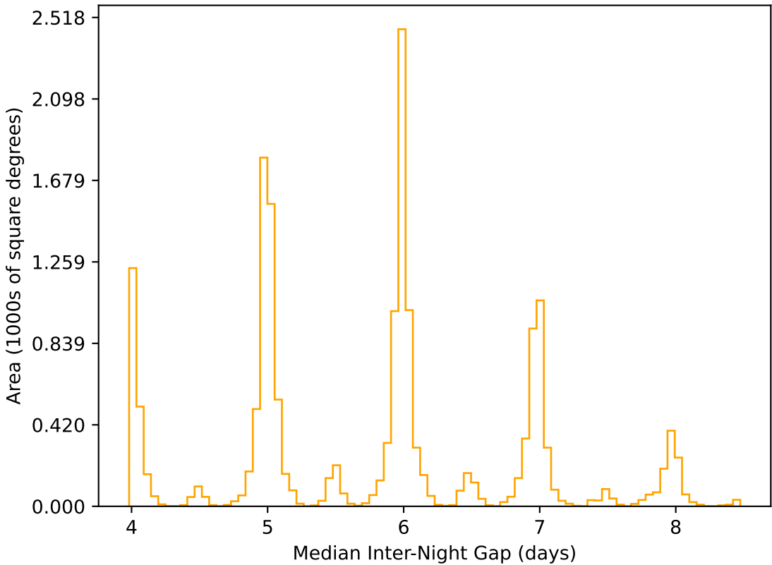
too_ignore_5_4v3.4_10yrs WFD r band: Median Inter-Night Gap
