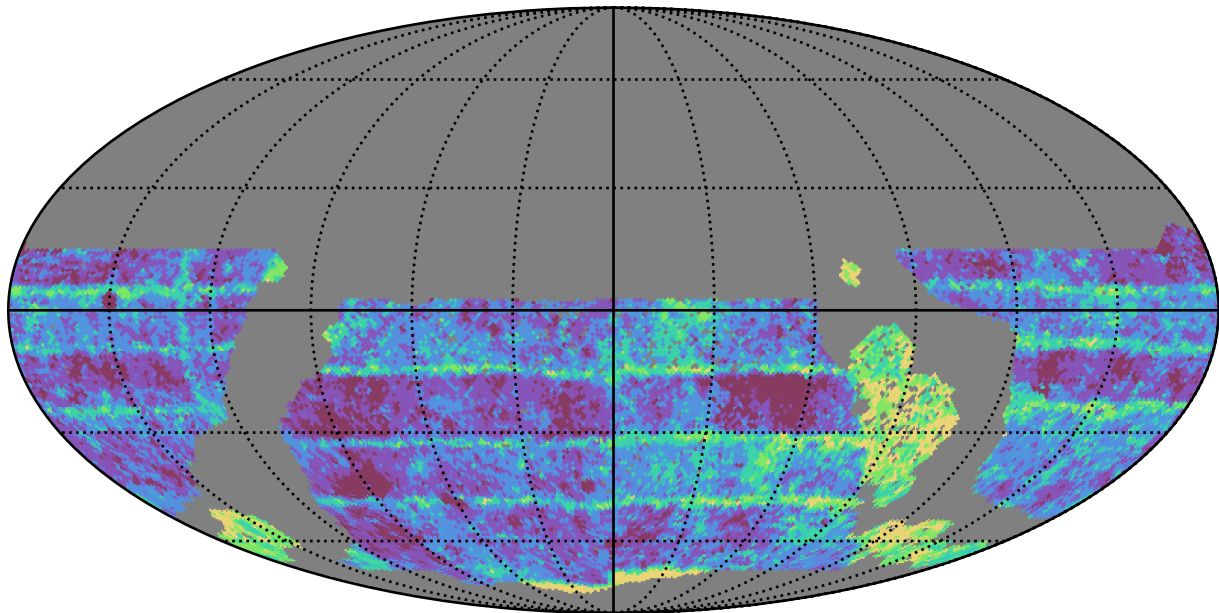
too_ignore_5_4v3.4_10yrs WFD i band: Median Inter-Night Gap
