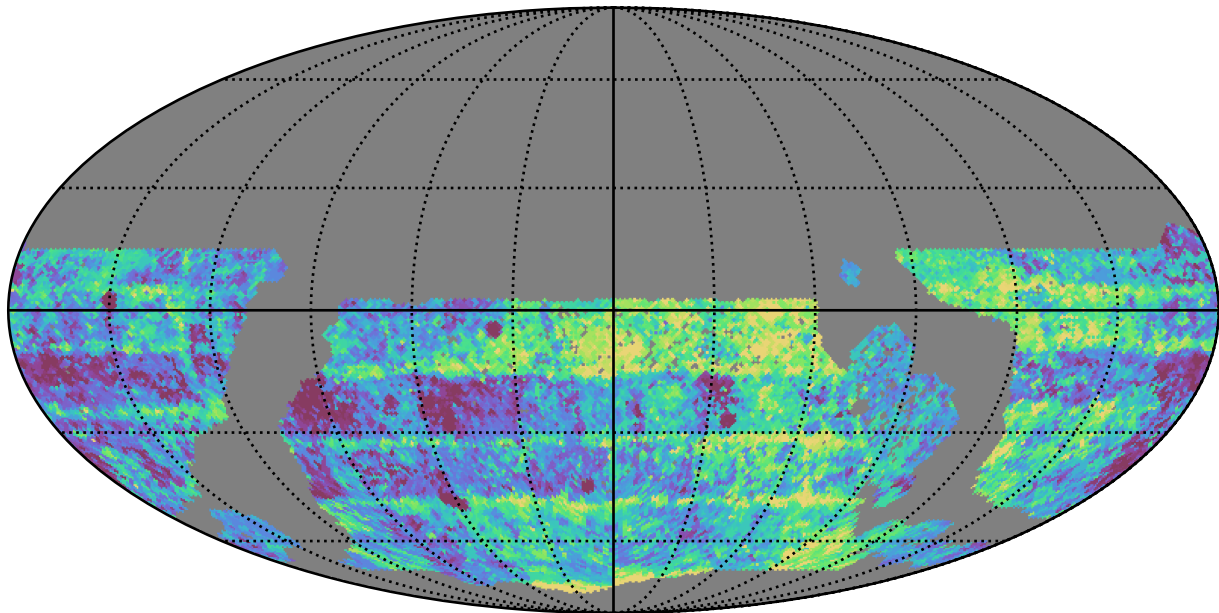
too_ignore_5_4v3.4_10yrs WFD g band: Median Inter-Night Gap
