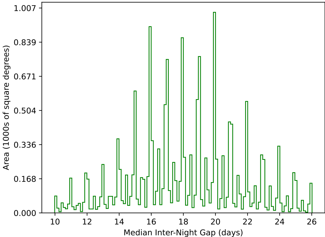
too_ignore_5_4v3.4_10yrs WFD g band: Median Inter-Night Gap
