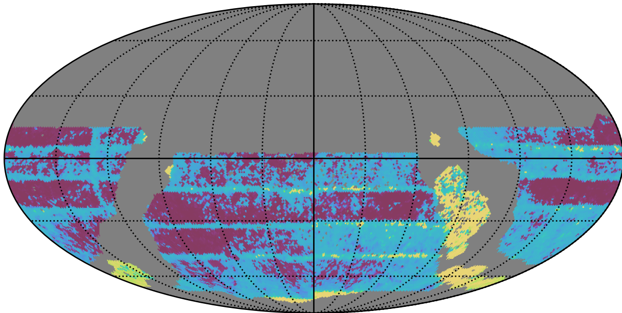
too_ignore_5_4v3.4_10yrs WFD all bands: Median Inter-Night Gap
