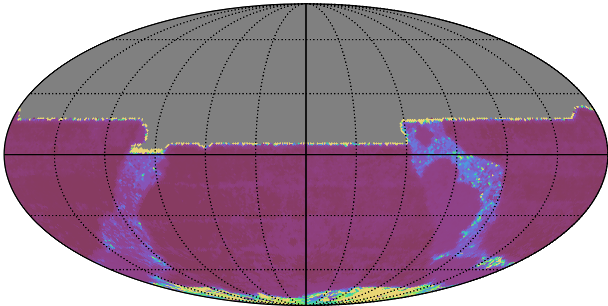
too_ignore_5_4v3.4_10yrs All sky y band: Median Inter-Night Gap
