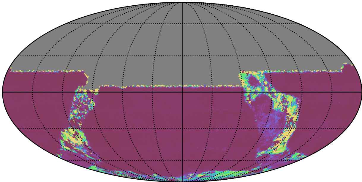
too_ignore_5_4v3.4_10yrs All sky u band: Median Inter-Night Gap
