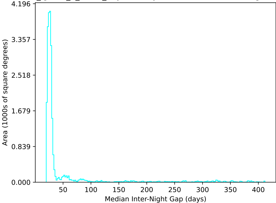
too_ignore_5_4v3.4_10yrs All sky u band: Median Inter-Night Gap
