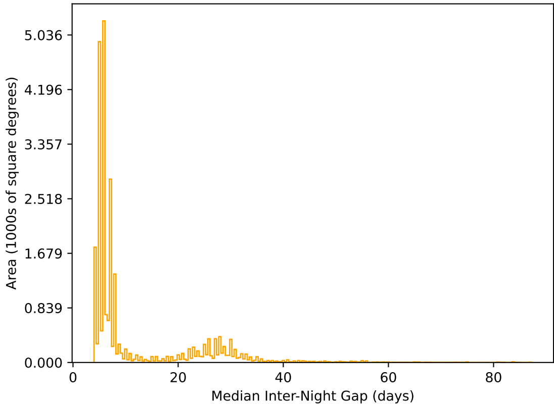
too_ignore_5_4v3.4_10yrs All sky r band: Median Inter-Night Gap
