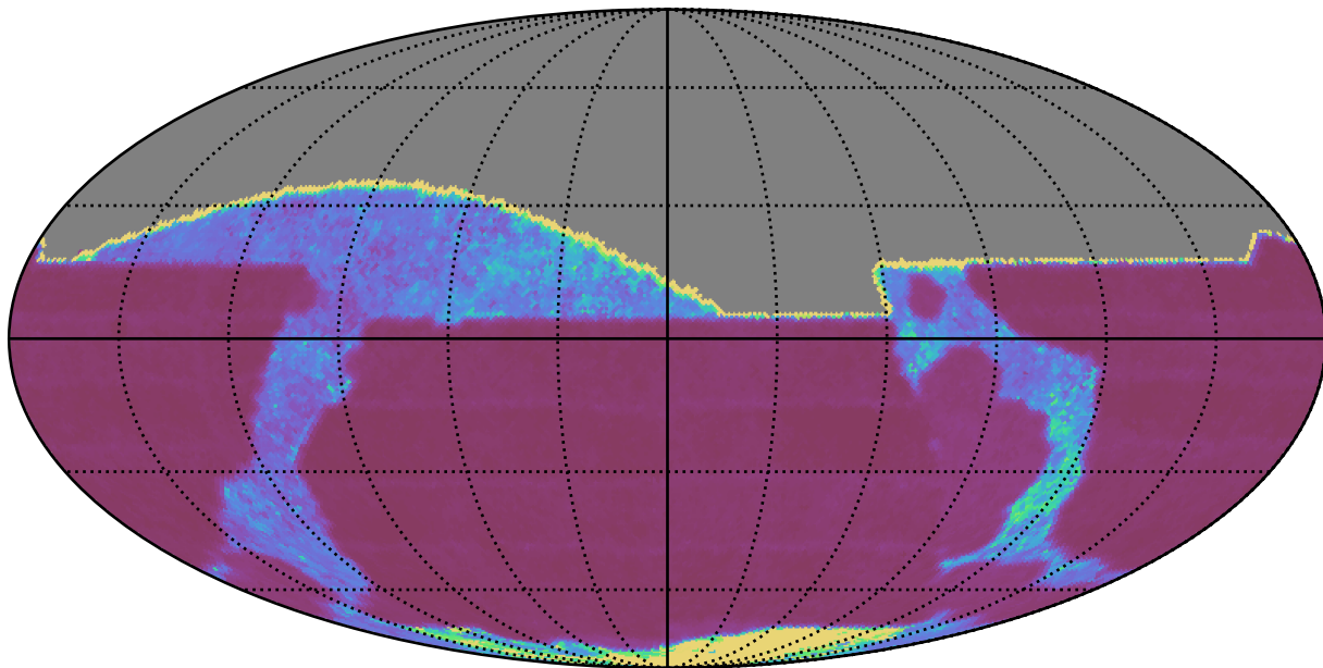
too_ignore_5_4v3.4_10yrs All sky i band: Median Inter-Night Gap
