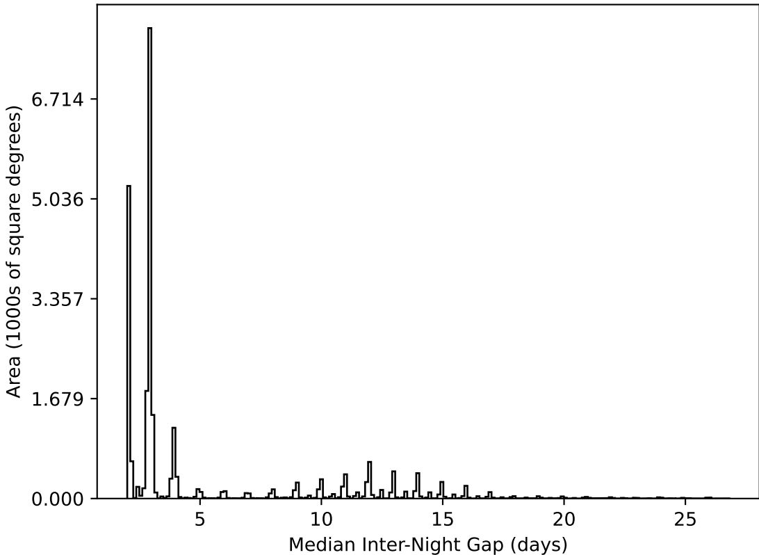
too_ignore_5_4v3.4_10yrs All sky all bands: Median Inter-Night Gap
