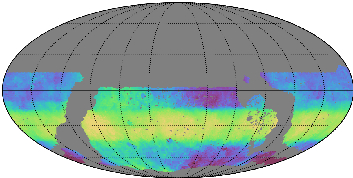
too_ignore_5_4v3.4_10yrs WFD z band: Median HA
