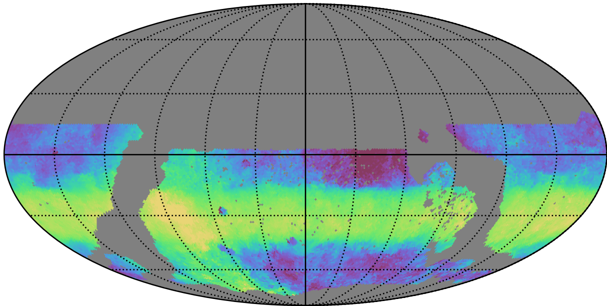
too_ignore_5_4v3.4_10yrs WFD y band: Median HA
