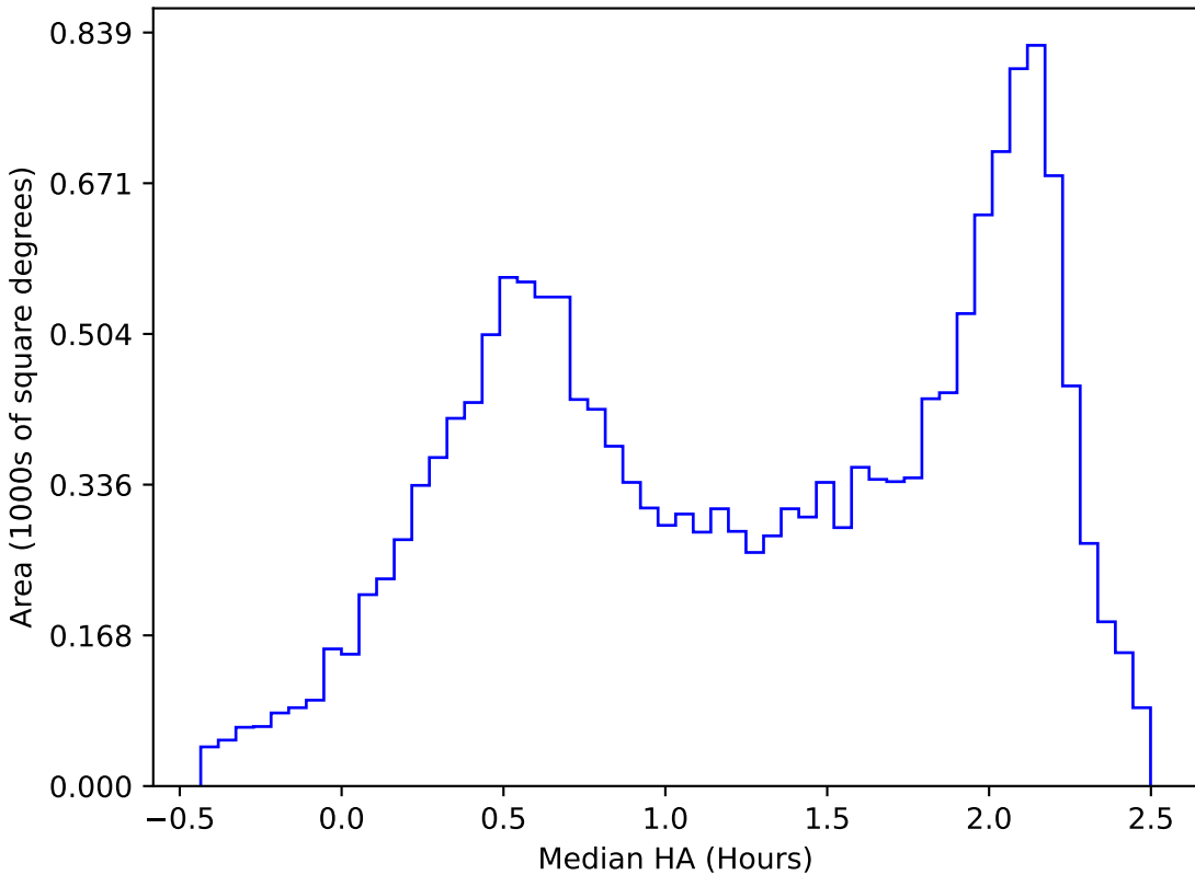
too_ignore_5_4v3.4_10yrs WFD y band: Median HA
