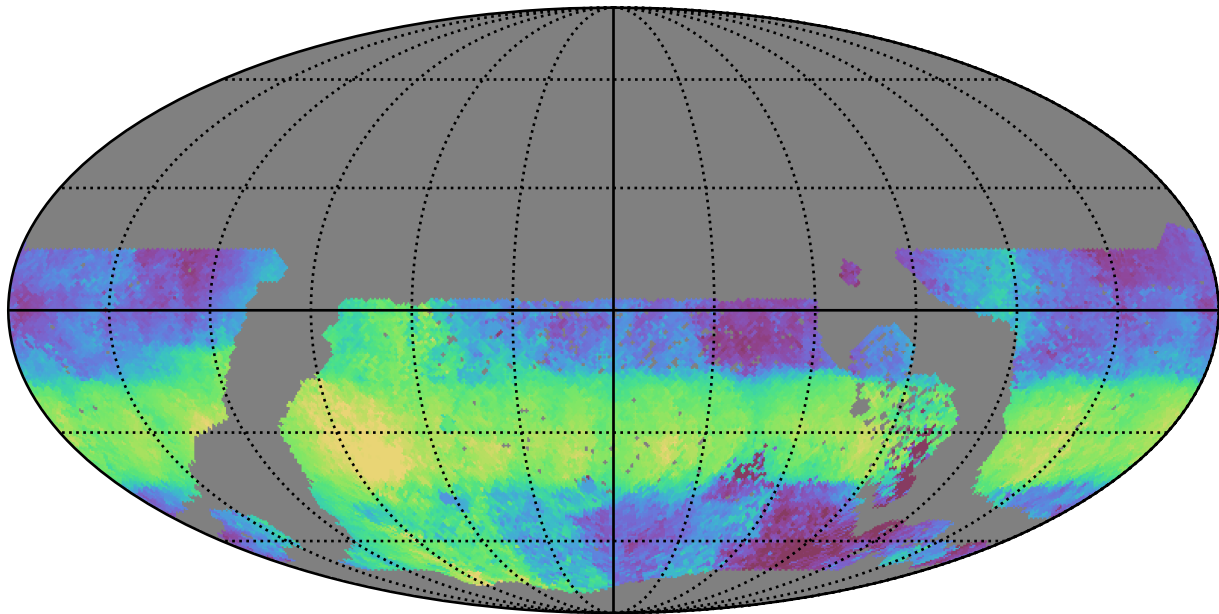
too_ignore_5_4v3.4_10yrs WFD u band: Median HA
