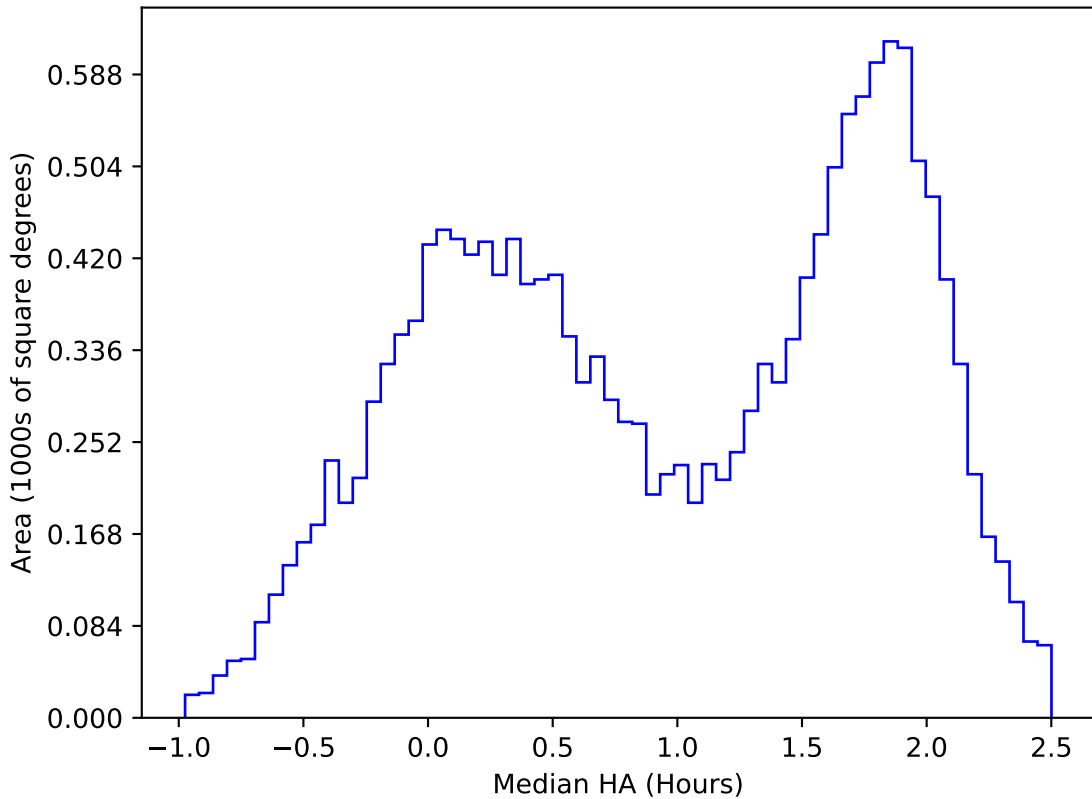
too_ignore_5_4v3.4_10yrs WFD u band: Median HA
