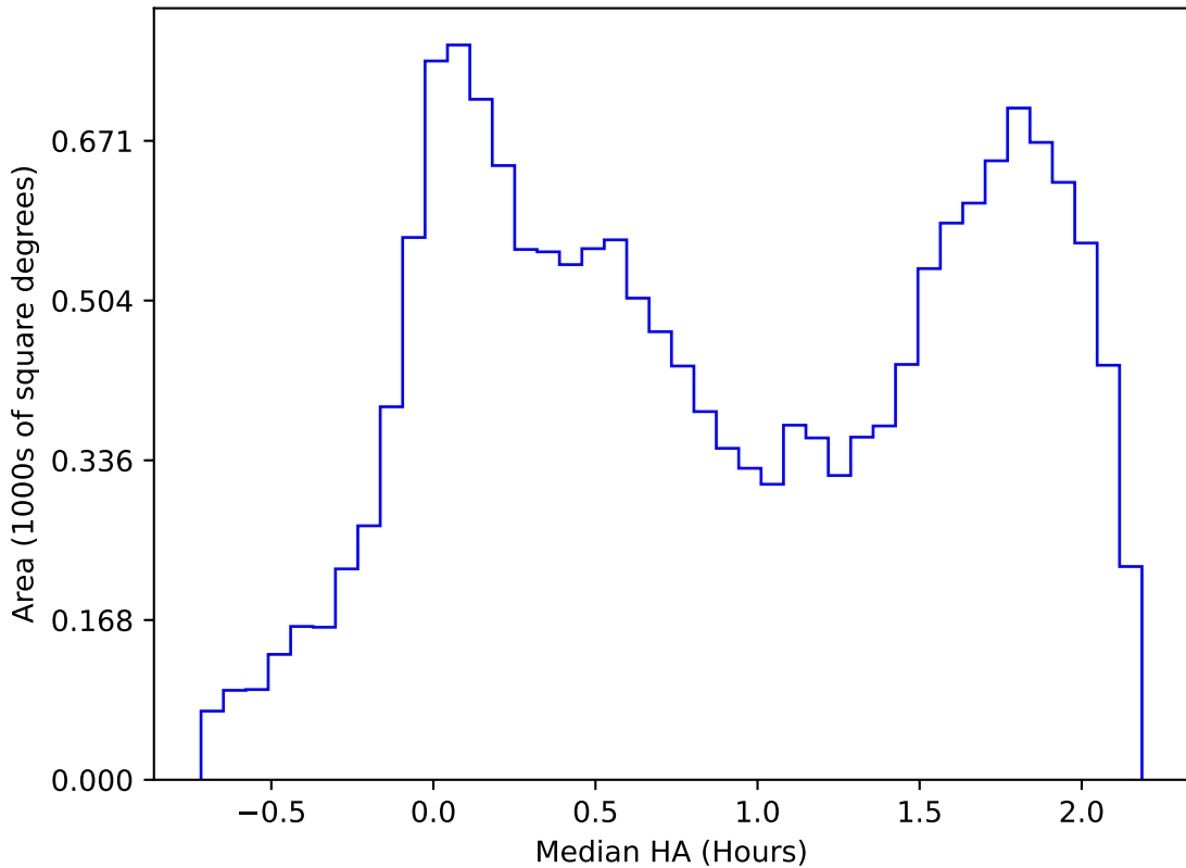
too_ignore_5_4v3.4_10yrs WFD r band: Median HA
