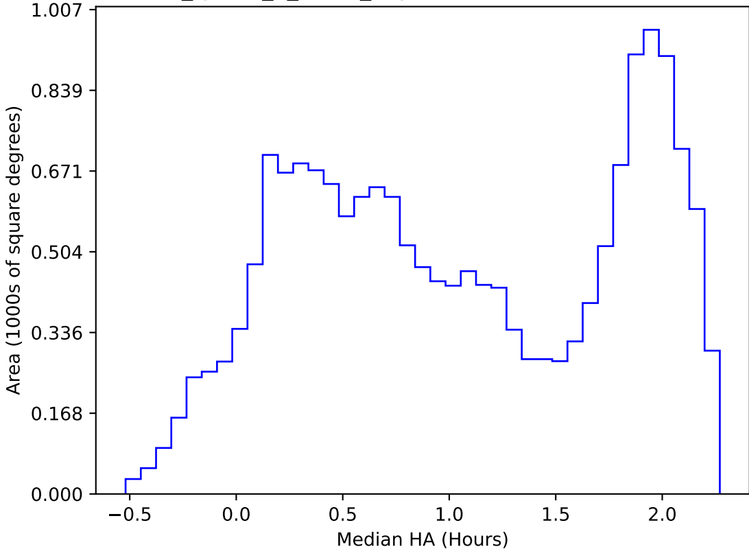
too_ignore_5_4v3.4_10yrs WFD i band: Median HA
