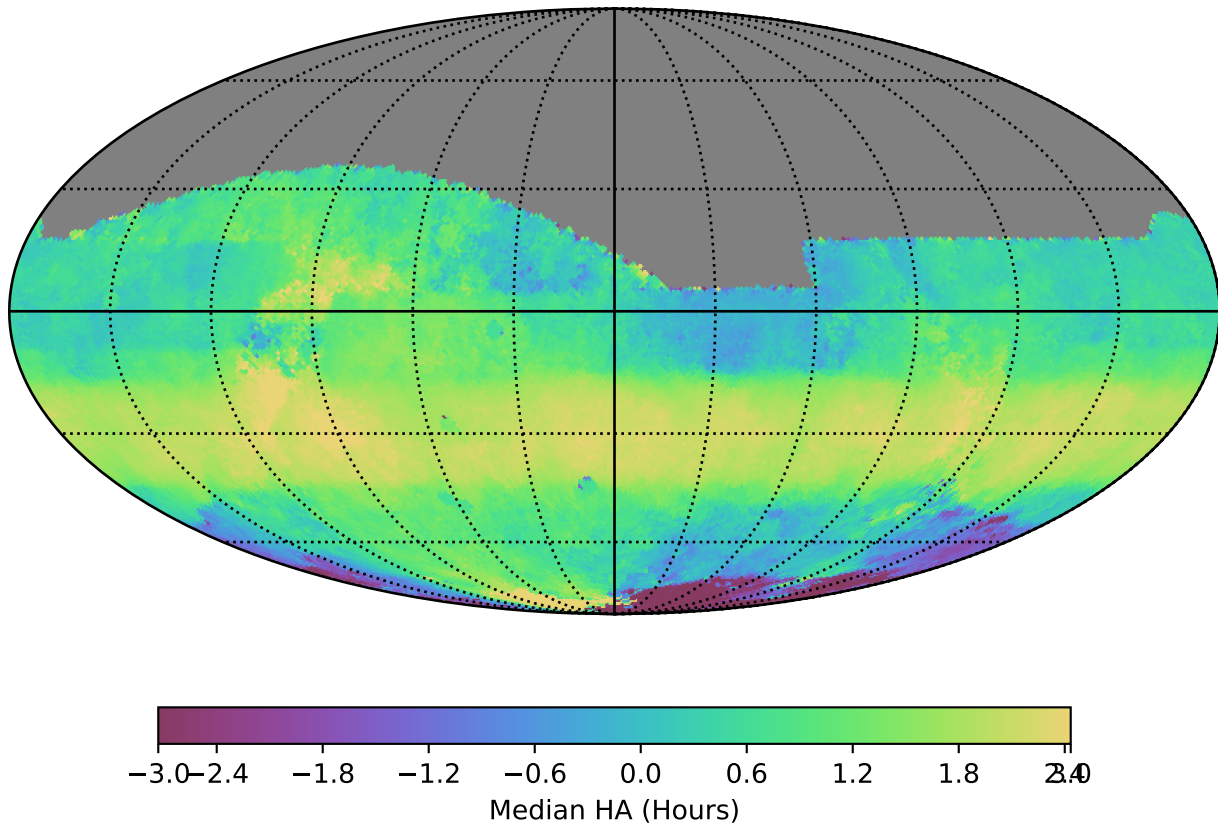
too_ignore_5_4v3.4_10yrs All sky z band: Median HA
