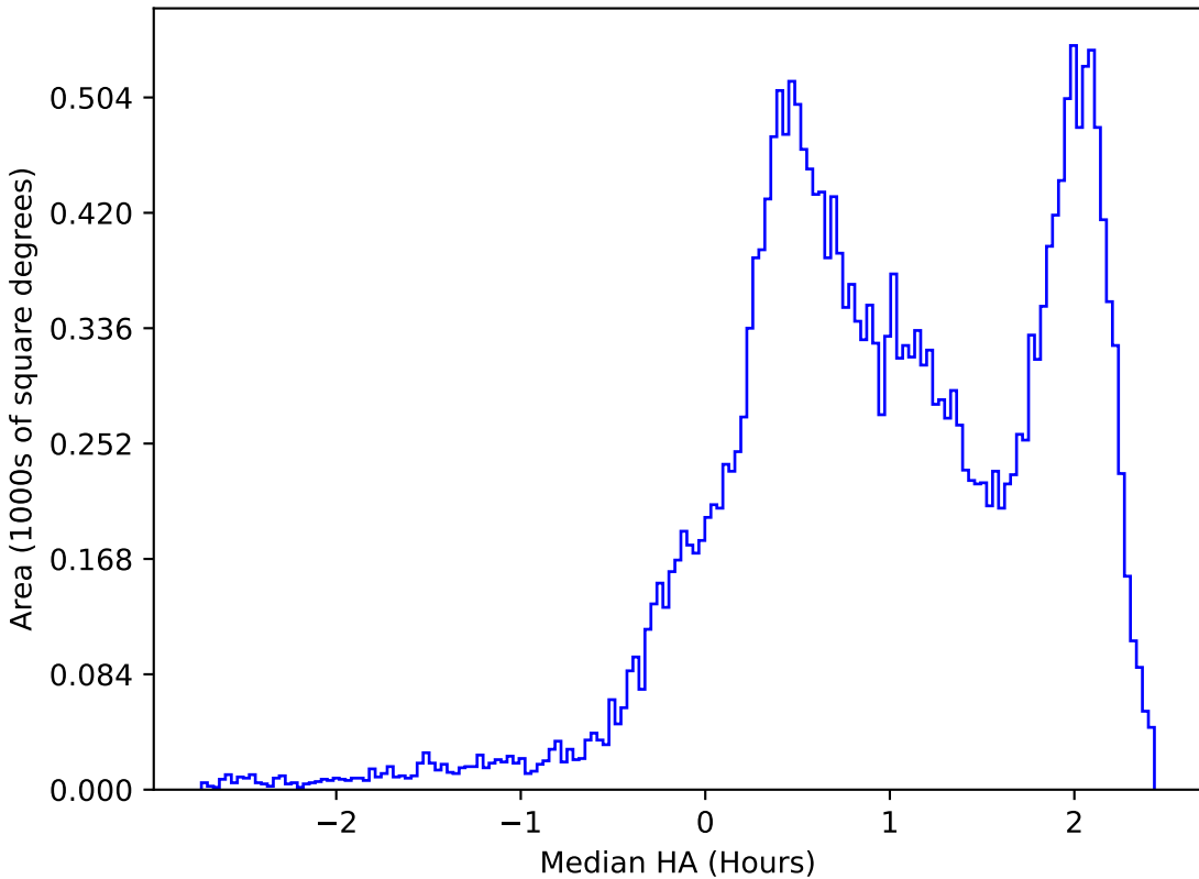
too_ignore_5_4v3.4_10yrs All sky z band: Median HA
