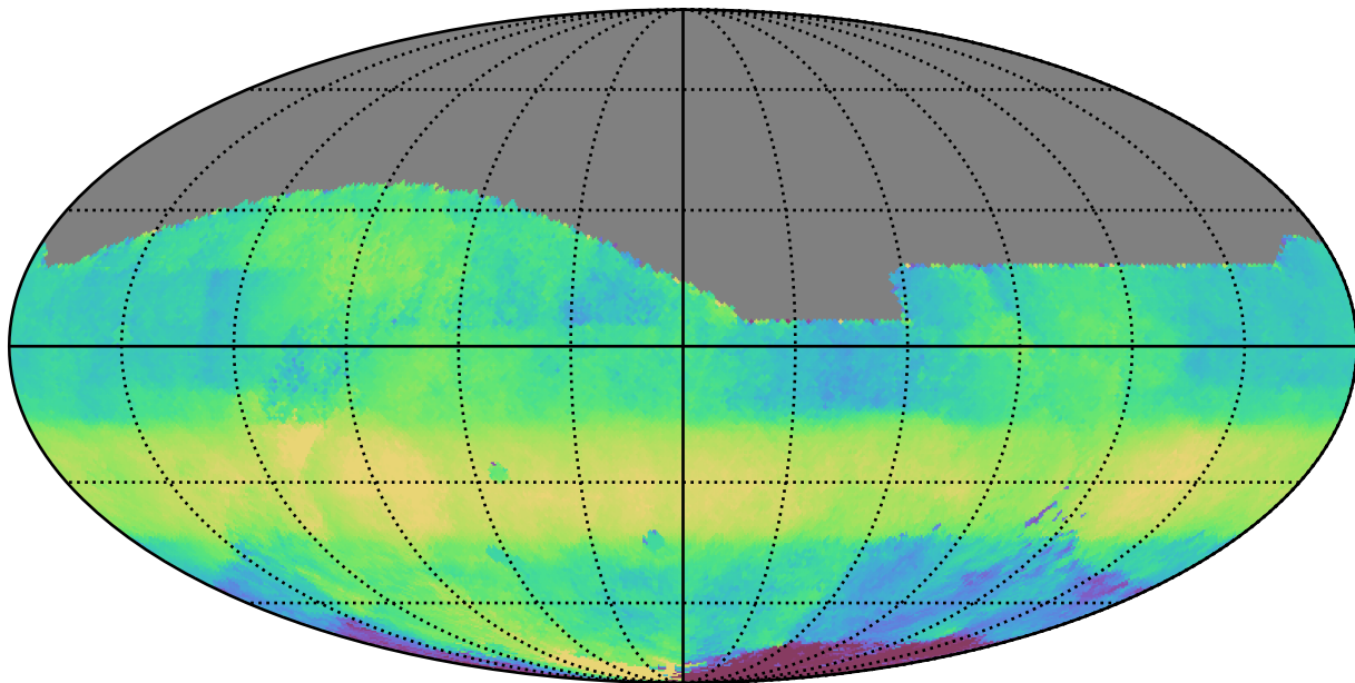
too_ignore_5_4v3.4_10yrs All sky r band: Median HA
