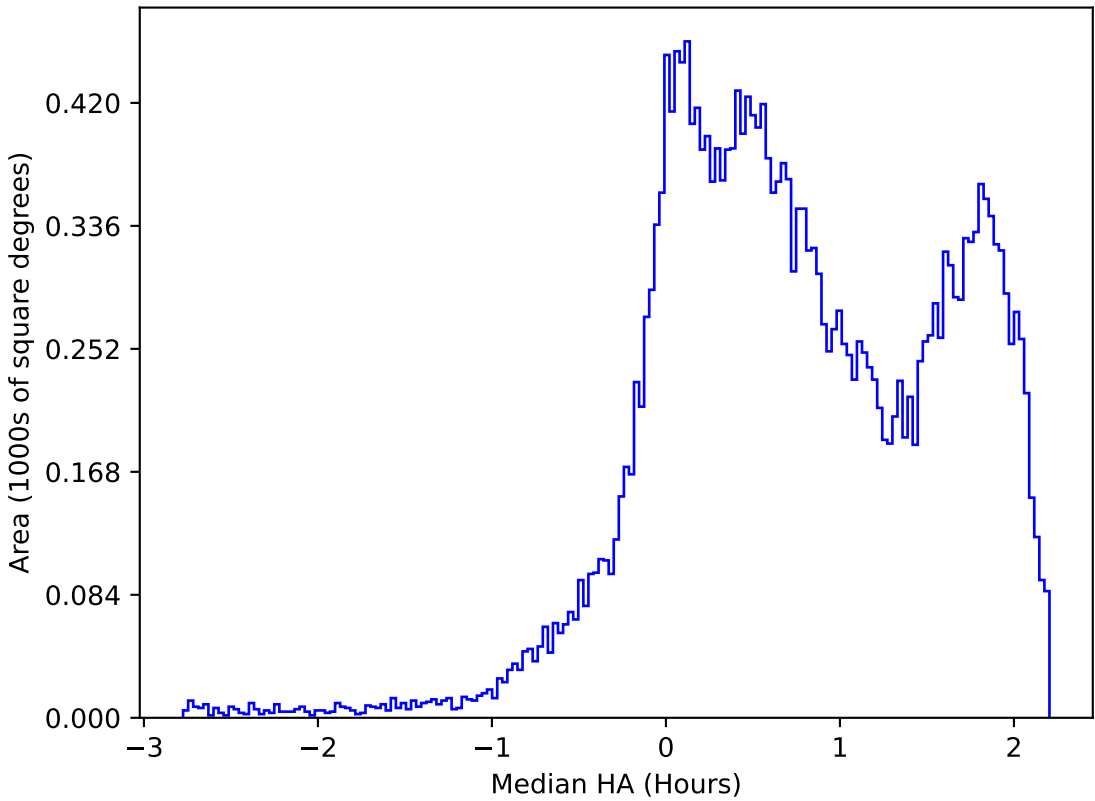
too_ignore_5_4v3.4_10yrs All sky r band: Median HA
