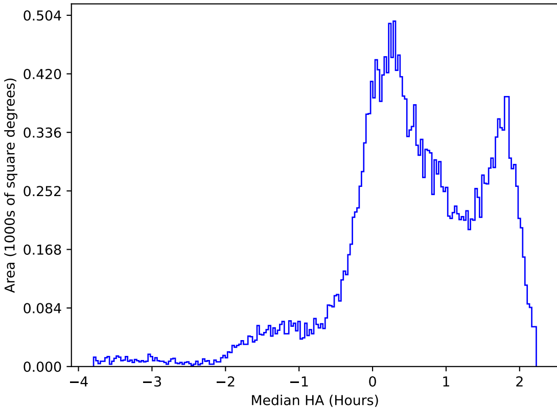
too_ignore_5_4v3.4_10yrs All sky g band: Median HA
