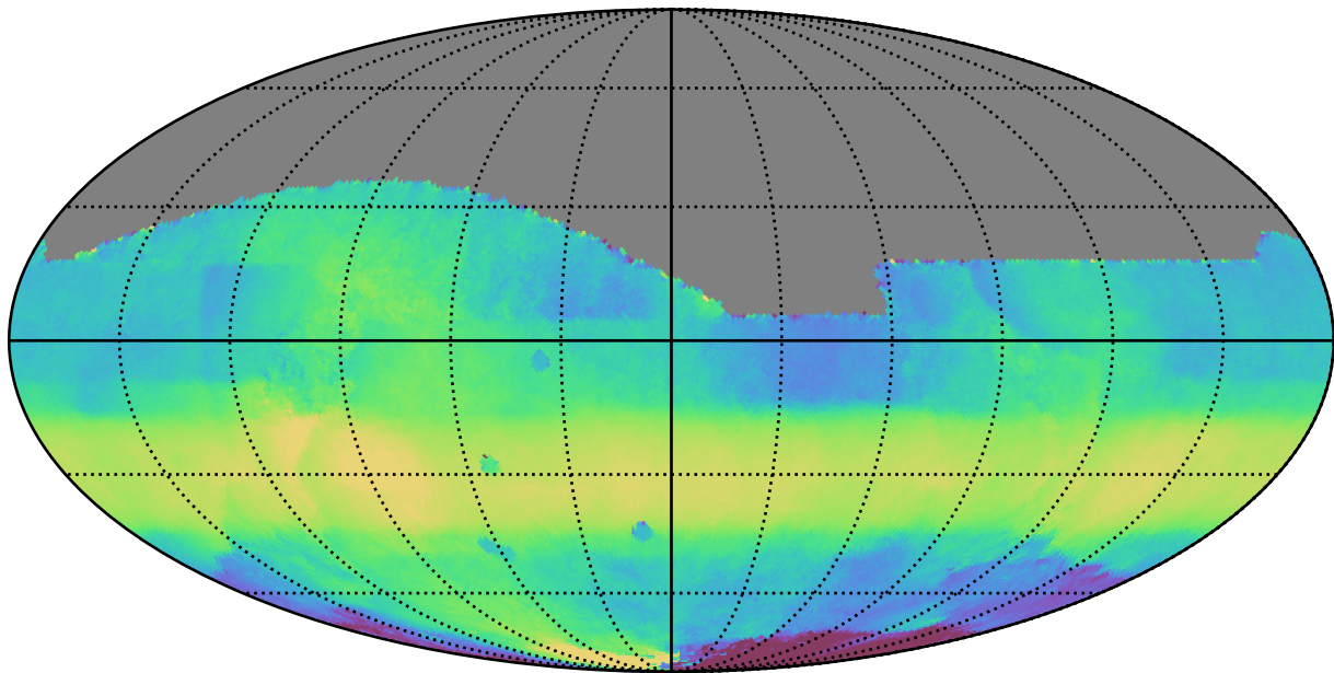
too_ignore_5_4v3.4_10yrs All sky all bands: Median HA
