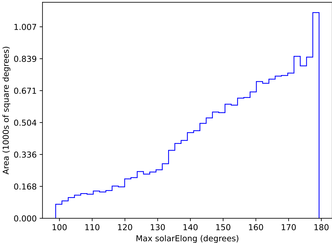
too_ignore_5_4v3.4_10yrs WFD z band: Max solarElong
