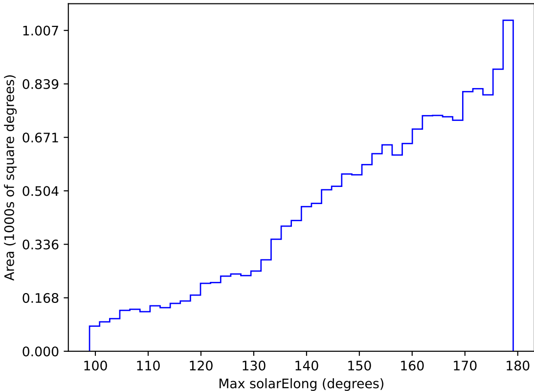
too_ignore_5_4v3.4_10yrs WFD y band: Max solarElong
