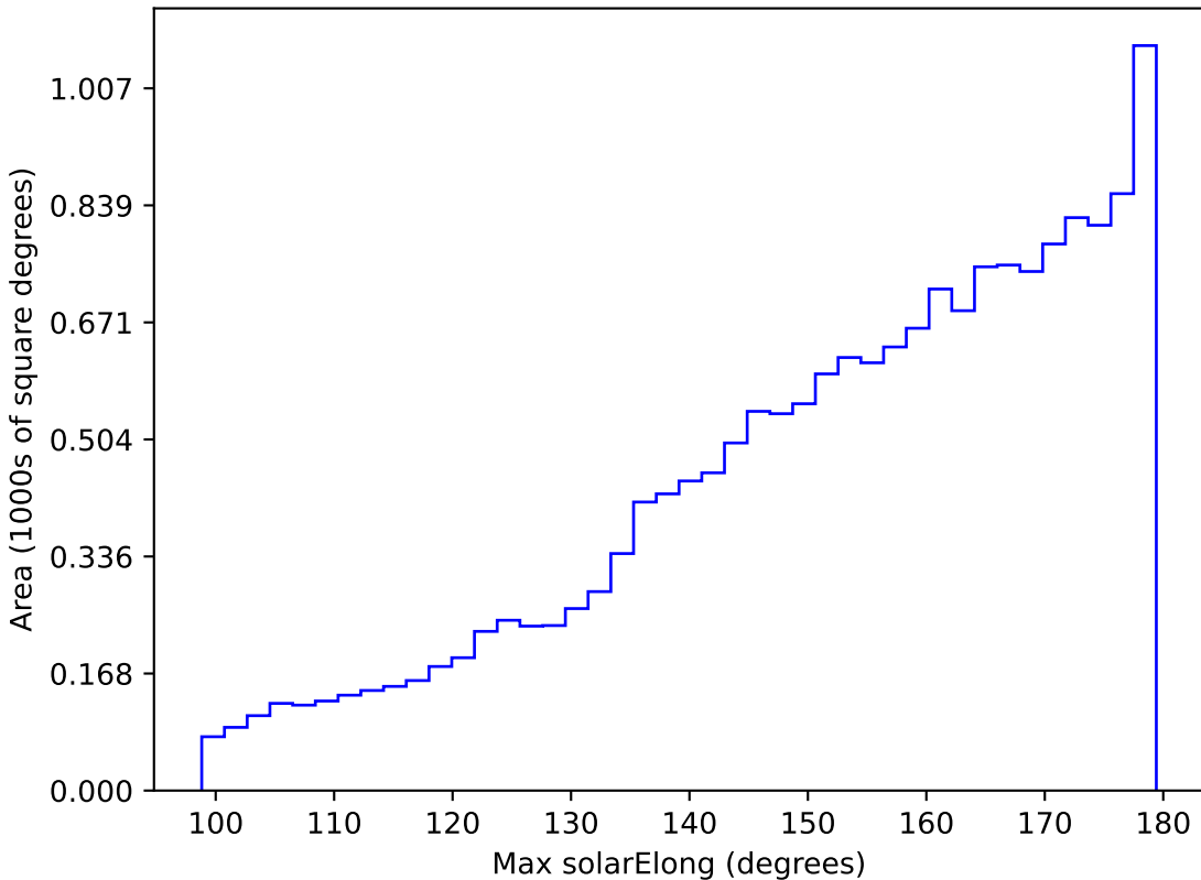
too_ignore_5_4v3.4_10yrs WFD r band: Max solarElong
