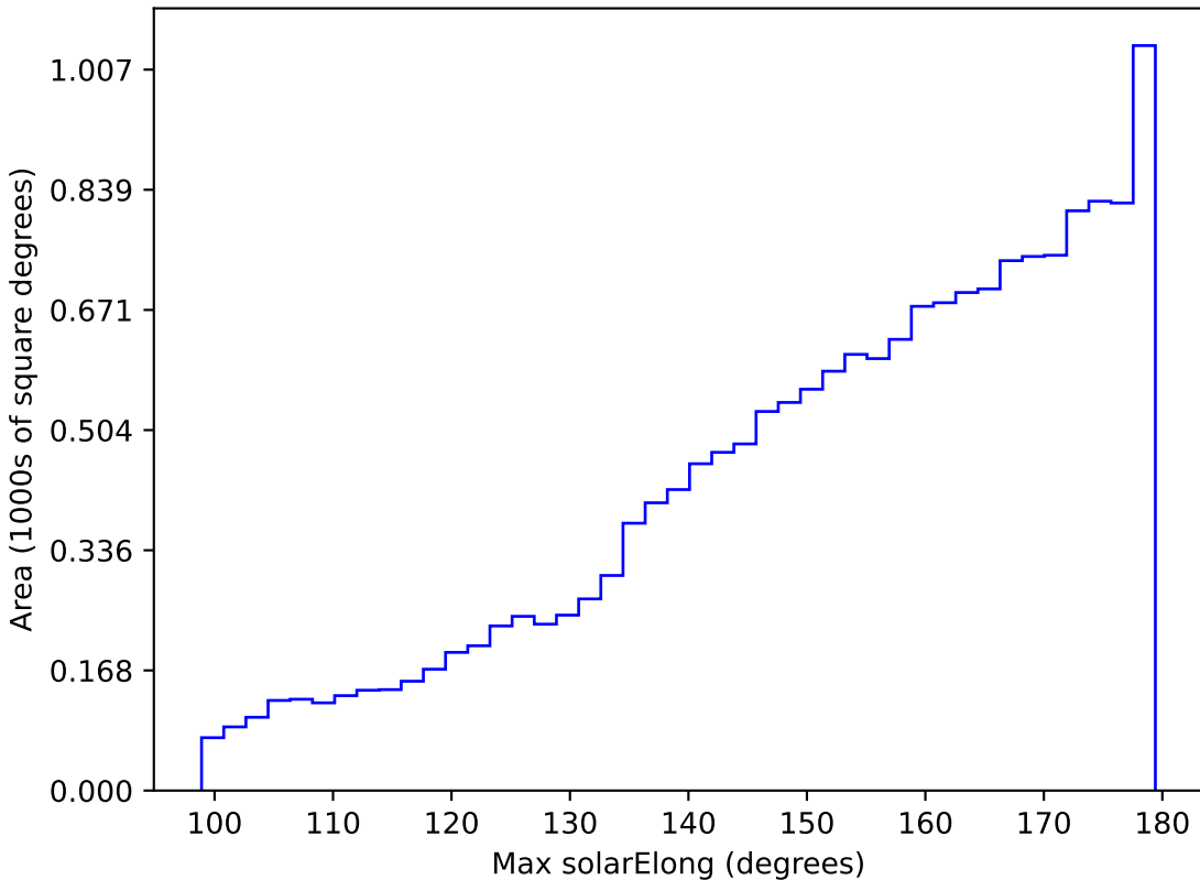
too_ignore_5_4v3.4_10yrs WFD i band: Max solarElong
