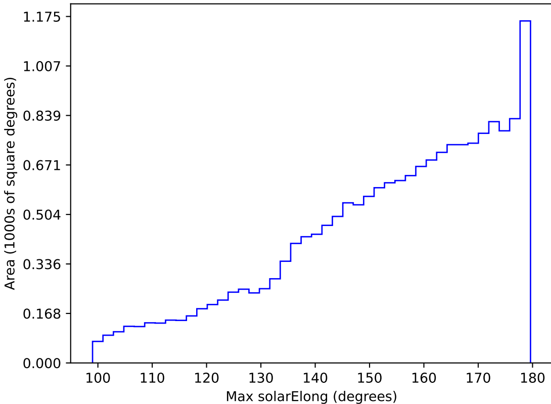
too_ignore_5_4v3.4_10yrs WFD all bands: Max solarElong
