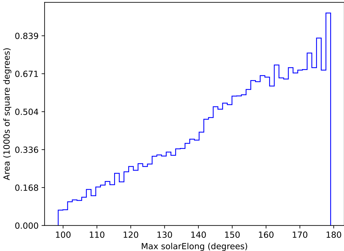
too_ignore_5_4v3.4_10yrs All sky y band: Max solarElong
