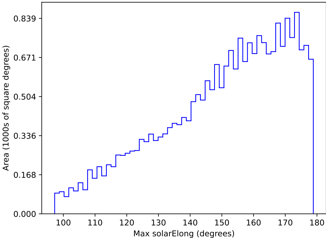
too_ignore_5_4v3.4_10yrs All sky u band: Max solarElong
